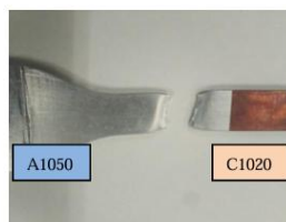
Fig.4 Fracture morphology of specimens after tensile test.
