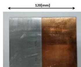
Fig.1 A1050 / C1020 dissimilar materials FSWed joint.
