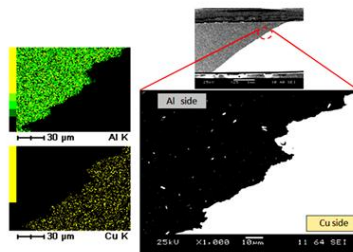
Fig.2 SEM observation of cross section in A1050/C1020 dissimilar materials FSWed joint.
