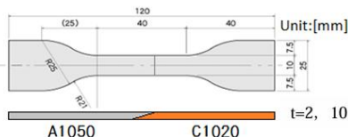
Fig.3 Geometry of joint specimen for tensile
